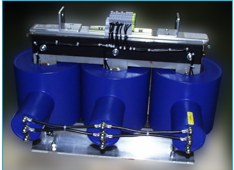
HTS 3000 - 50 3p Three phase version
