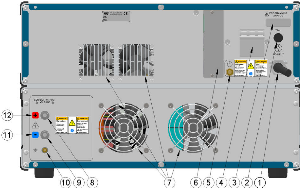
Figure: Sample MCP 5000 – 2000. For DC power supplies with higher performance or other voltages, other dimensions may apply. The arrangement of the elements may be different from that, shown here.
