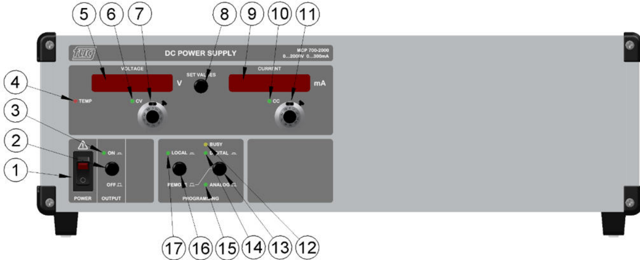
Figure: Sample Front panel MCP 700 – 2000. Different dimensions apply for DC power supplies with higher performance
